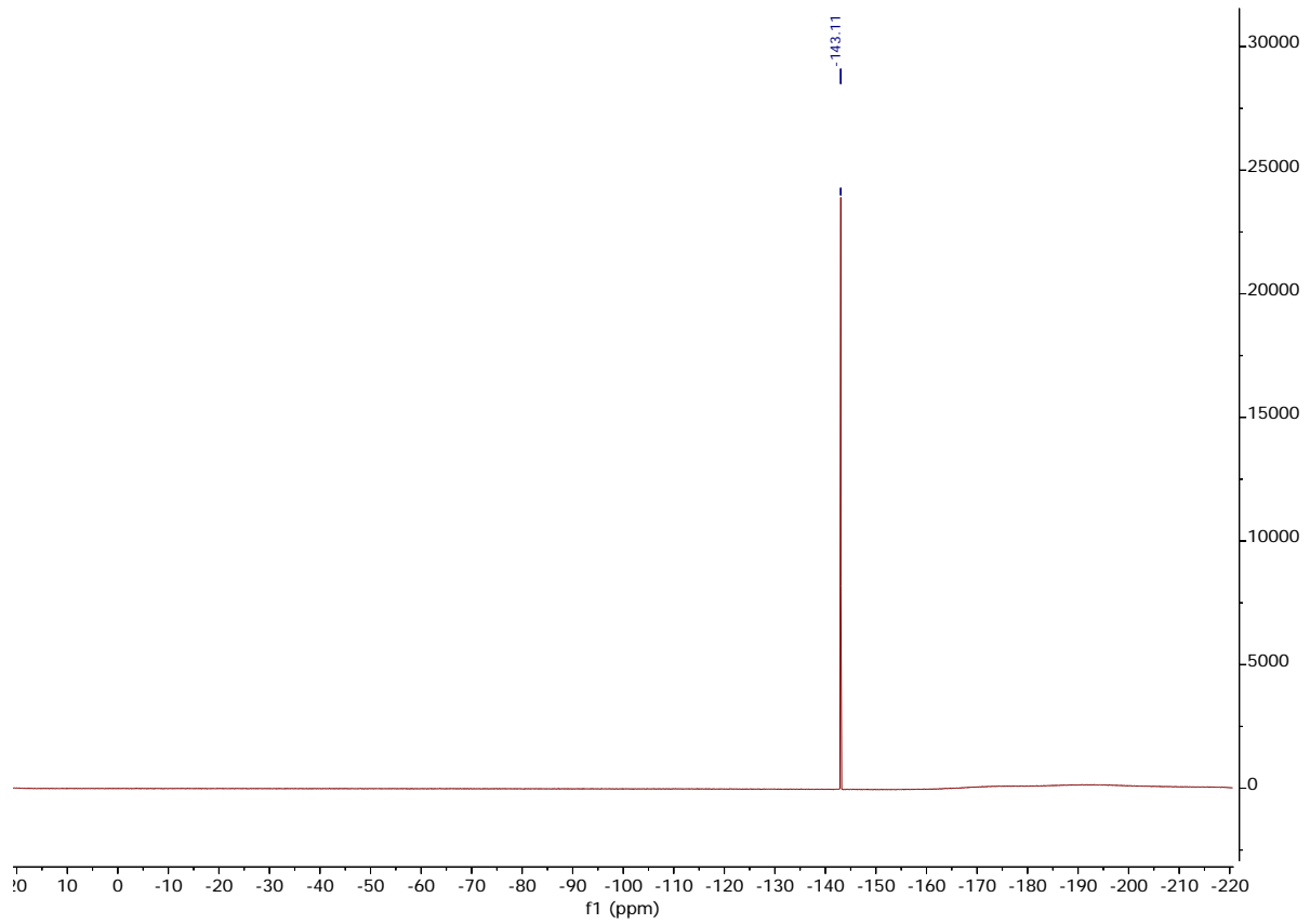
^{19}\text{F} -NMR Spectrum 470 MHz ( \text{CDCl}_3 , 25 °C)
